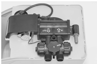
Diagram 12: Bypass Position
