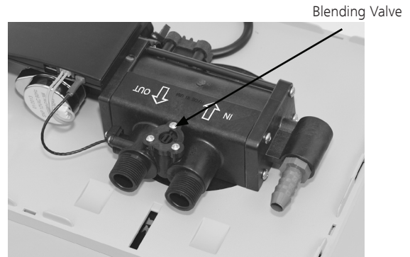
Diagram 18: Adjusting Blending Valve
