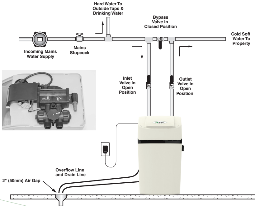
Diagram 13: Service Position
